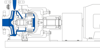
Frame-mounted MSKP with baseplate -20°C to +100°C
