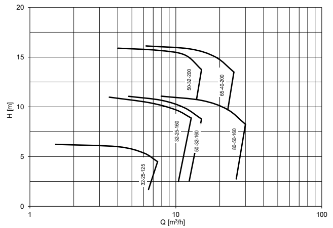
1500 rpm/50 Hz
