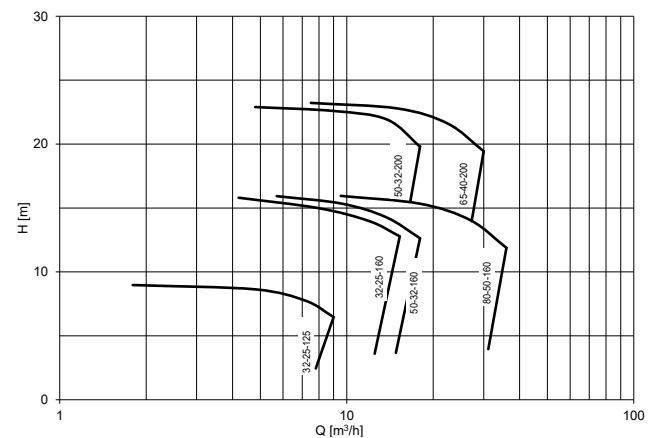
1800 rpm/60 Hz
