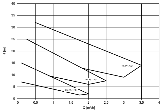
1500 rpm/50 Hz
