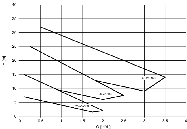
1500 min -1 /50 Hz
