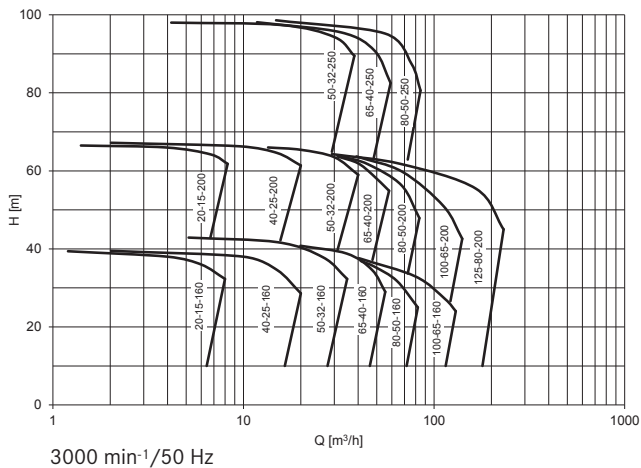
3000 min -1 /50 Hz
