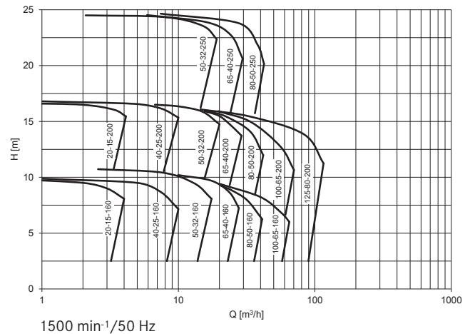
1500 min -1 /50 Hz
