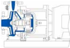
Close-coupled MSKP with baseplate -4 °F to +212 °F
