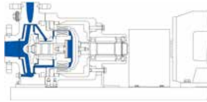
Frame-mounted MSKP with baseplate -4 °F to +212 °F
