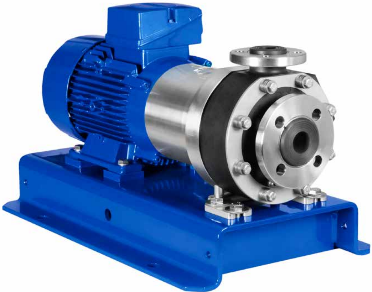
MSKP with baseplate and motor horizontal close-coupled (-4 °F to +212 °F)
