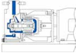
Close-coupled MSKPP with baseplate -4 °F to +212 °F
