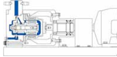
Frame-mounted MSKPP with baseplate -4 °F to +212 °F
