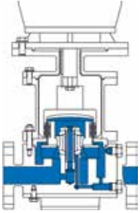
Vertical in-line close-coupled SZMK with stand -148°F to +392°F
