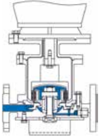
Vertical in-line close-coupled MKPP with stand -148°F to +392°F
