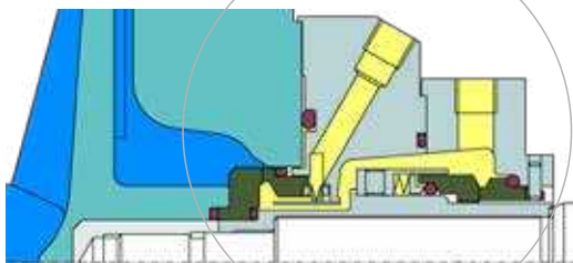
FuturaMik® double mechanical seal
