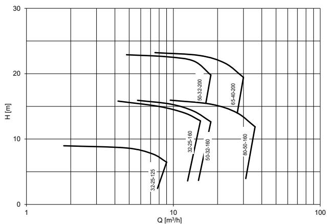
1800 rpm/60 Hz
