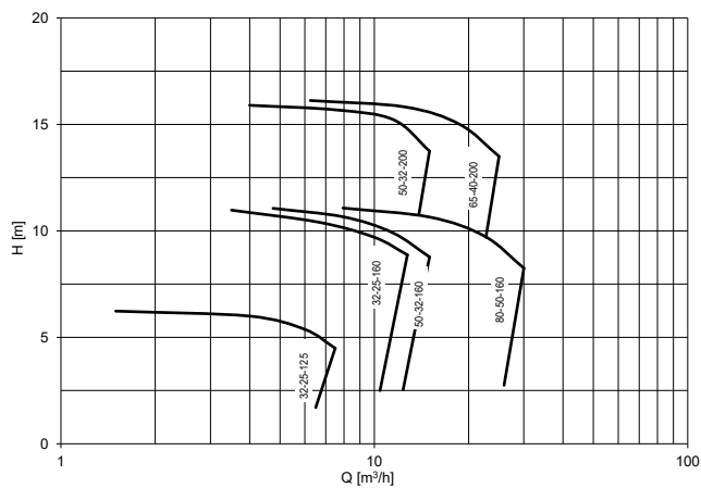
1500 rpm/50 Hz
