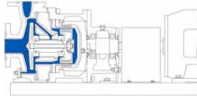
Bearing frame-mounted MKPL with baseplate -4 to +392°F
