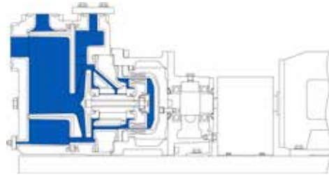
Bearing frame mounted MKPL-S with baseplate -4 to +302°F
