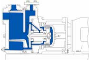
Close-coupled MKPL-S with baseplate -4 to +302°F
