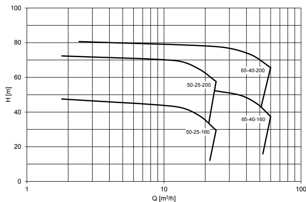
3600 rpm/60 Hz
