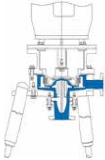
Close-coupled MKP-Bio with tripod -4 °F bis +302 °F
