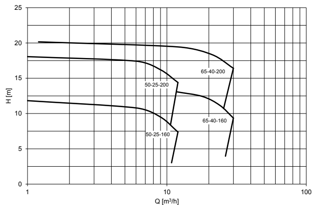
1800 rpm/60 Hz
