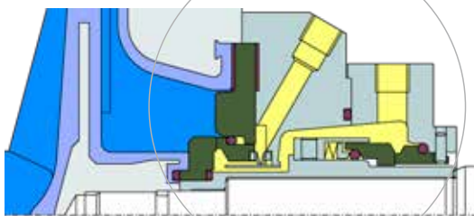
FuturaTef® double mechanical seal
