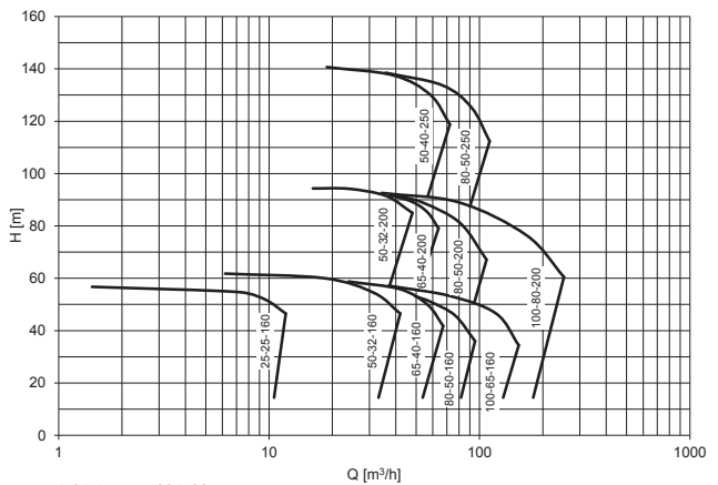
3600 rpm/60 Hz
