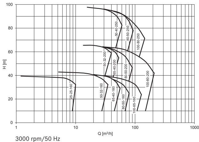
3000 rpm/50 Hz
