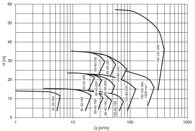
1800 rpm/60 Hz
