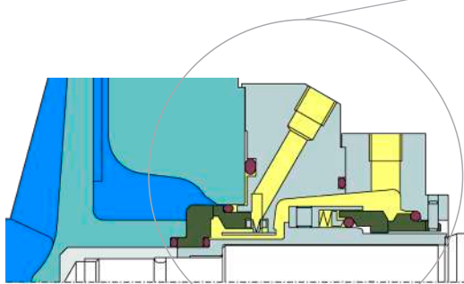
FuturaMik® double mechanical seal
